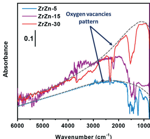
Fig. 2 FT-IR difference spectra of ZrZn-X catalysts at 400 °C in H_2 (subtrahend spectrum is that recorded in oxygen at 400 °C). The ZrZn-5 spectrum is cut at 3155\text{ cm}^{-1} because, beyond that frequency, data are affected by the low signal-to-noise ratio; the cut part has been substituted with a dotted blue line, which aims to reproduce the trend.
