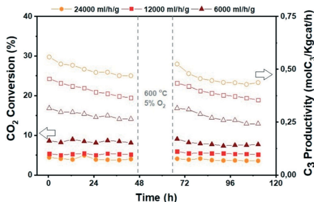
Fig. 11 Catalytic performance of the ZrZn-30/ZSM-5 combined system before and after regeneration for \text{CO}_2 conversion to hydrocarbons at different space times. \text{CO}_2 : \text{H}_2 1:3, 350 °C, 30 bar.
