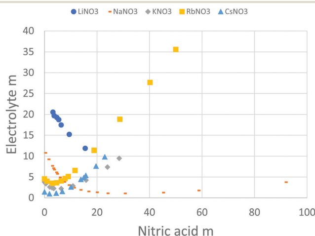
Fig. 9 Solubility of alkali nitrate salts in nitric acid at 25 °C. Data from ref. 19 and 32–34.
