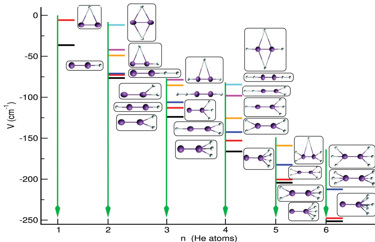
Fig. 7 Schematic representation of optimal low-lying structures and their energetics obtained using the sum-of-potential He n-1-6 K 2 + PESs.
