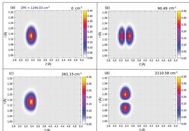
Fig. 8 2D \rho(Z, r) plots of selected 3D eigenfunctions, (a) ground state, (b) first “Z-excited” state, (c) first “ \theta -excited” state, (d) first “ r -excited” state, of 1/4 ML P/U CO:NaCl(100) along Z and r , at \theta = 0.9^\circ , obtained from BIR-MCTDH. Energies are relative to the ground state.
