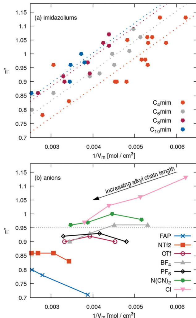
Fig. 5 Kamlet-Taft \pi^* -values as a function of inverse molar volume. (a) Restricting the set of ILs to a particular C_nmim . (b) Fixing the anion and follow the trend with increasing chain length of the imidazolium.
