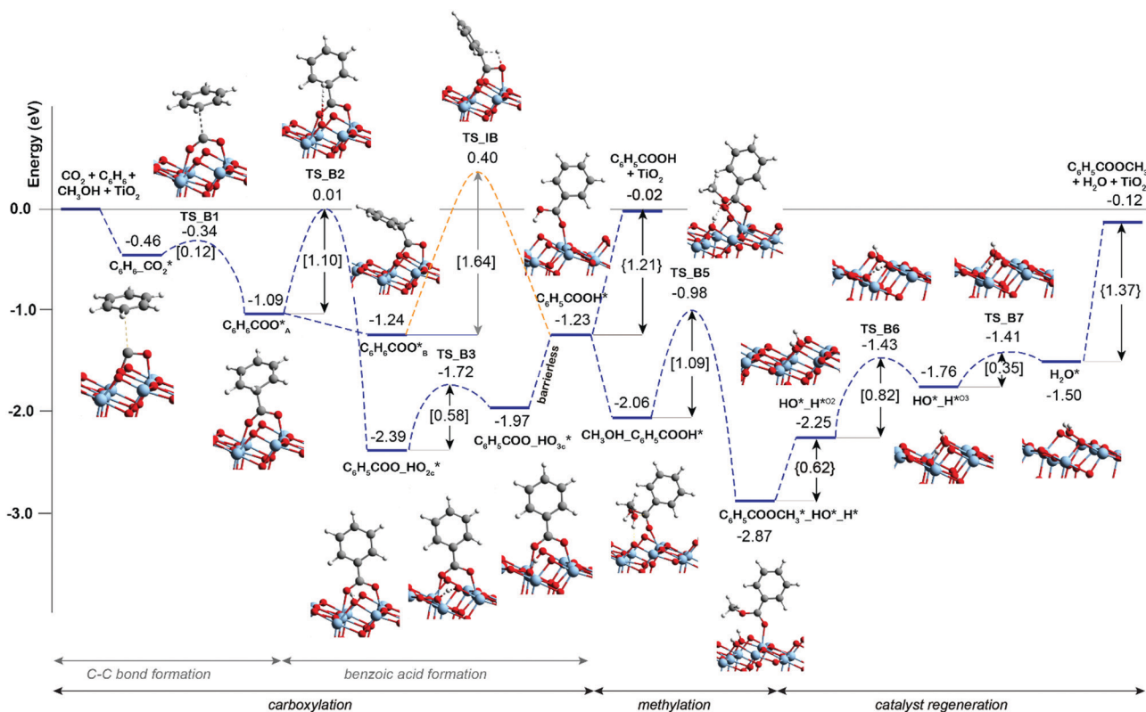
Fig. 2 Reaction energy diagram for the benzene esterification with \text{CO}_2 and \text{CH}_3\text{OH} on defective \text{TiO}_2 surface.
