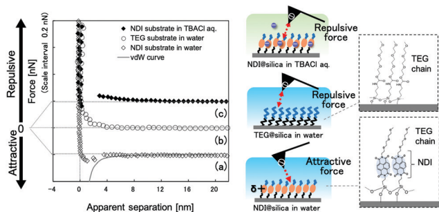
Fig. 4 Approaching force curves of NDI@silica in pure water (a), TEG@silica substrate in pure water (b), and NDI@silica in 10 mM TBACl aqueous solution (c). The theoretical curve of van der Waals force is attached on the curve of NDI@silica in pure water. The Z-scale interval is 0.2 nN.
