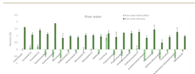
Fig. 2 SPE recovery and matrix effect of antifungal agents in river water samples (a negative value indicates ionization suppression and a positive value indicates ionization enhancement).
