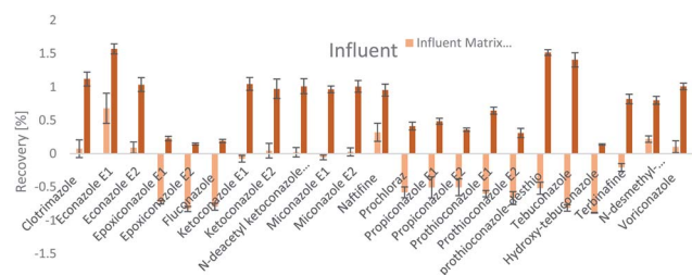
Fig. 4 SPE recovery and matrix effect of antifungal agents in influent samples (a negative value indicates ionization suppression and a positive value indicates ionization enhancement).
