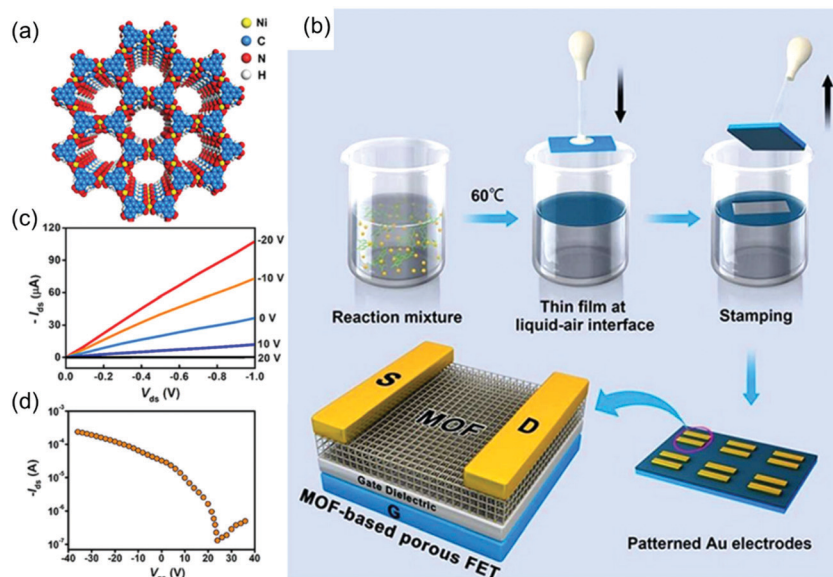
Fig. 15 (a) Schematic structure of semiconducting \text{Ni}_3(\text{HITP})_2 . (b) Schematic illustration of the fabrication of \text{Ni}_3(\text{HITP})_2 film-based porous FETs. (c and d) Output curves and transfer curve for the \text{Ni}_3(\text{HITP})_2 -based FET, respectively. Reproduced with permission from ref. 164. Copyright 2017 American Chemical Society.
