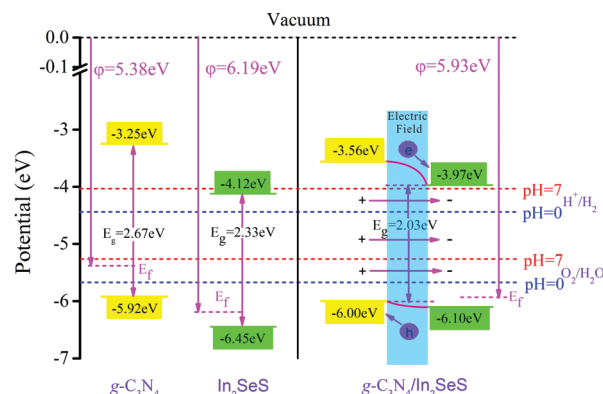
Fig. 6 Potential of band-edge positions for \text{g-C}_3\text{N}_4 , monolayer \text{In}_2\text{SeS} and the \text{In}_2\text{SeS/g-C}_3\text{N}_4 heterostructure.
