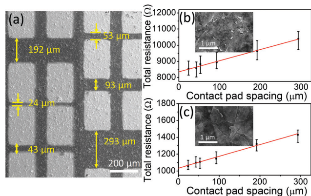
Fig. 4 SEM image of Au/Ti contact pads on \text{Ti}_3\text{C}_2\text{T}_x films on \text{SiO}_2/\text{Si} (a), plots of total resistance vs. contact pad spacing of (b) \text{Ti}_3\text{C}_2\text{T}_x and (c) r\text{-Ti}_3\text{C}_2\text{T}_x films on \text{SiO}_2/\text{Si} . Insets in figures b and c are the high magnification SEM images of the corresponding films.
