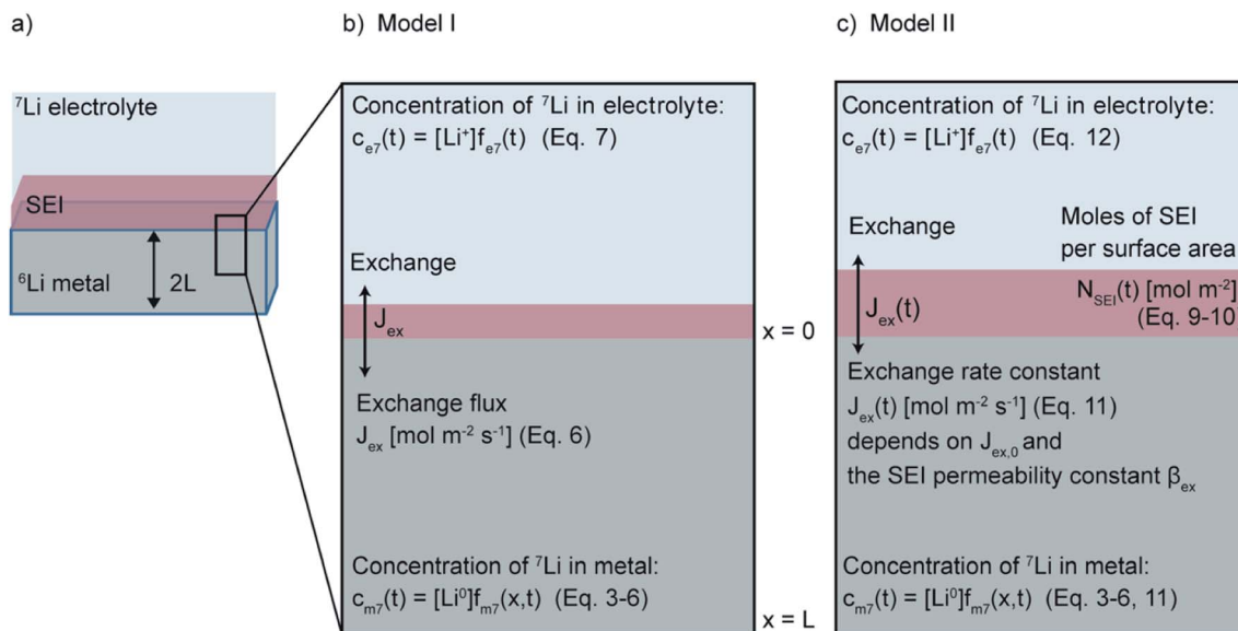
Fig. 1 A schematic showing (a) the geometry of the Li metal electrode, (b) Model I, which uses one fitting parameter, the isotope exchange flux, J_{ex} [mol m -2 s -1 ] to describe the isotope exchange and (c) Model II, which describes both isotope exchange and SEI formation, via J_{ex}(t) [mol m -2 s -1 ] that depends on the initial isotope exchange rate flux J_{ex,0} and the SEI permeability constant \beta_{ex} . The relevant equations and equation numbers describing the processes are indicated in the schematics.
