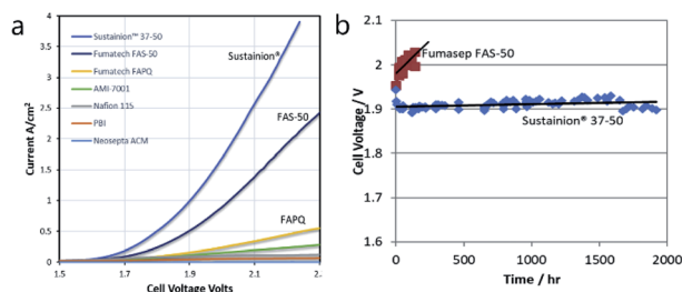
Fig. 9 (a) Comparison of current–voltage response of AEM electrolysis with various membranes in ref. 119. (b) Steady state voltage performance at 1 A cm -2 with Sustainion 37–50 membrane and FAS-50 membrane (60 °C, 1 M KOH, NiFe 2 O 4 anode and NiFeCo cathode). Reprinted from ref. 125 with permission from Elsevier. 125
