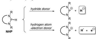
c) Consumption and regeneration of the catalyst NHP
