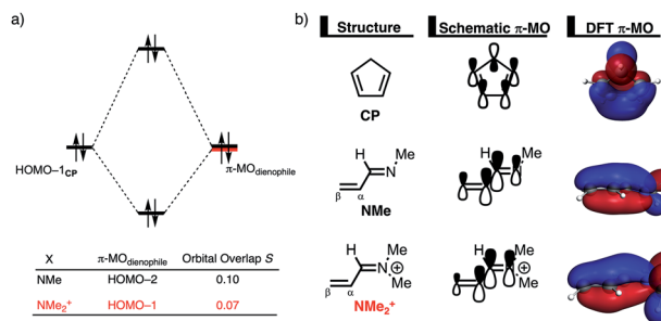
Fig. 4 Molecular orbital diagrams of the key orbital interactions of the Diels–Alder reactions between CP and NMe and NMe 2 + : (a) most significant occupied orbital overlaps and (b) 3D plots of the involved occupied orbitals (isovalue = 0.03 au −3/2 ). All data were computed at consistent geometries with a C CP ...C \beta bond length between CP and the dienophile of 2.125 Å at ZORA-M06-2X/TZ2P//M06-2X/def2-TZVP.
