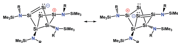
Fig. 6 Possible resonance structure of 2 .
