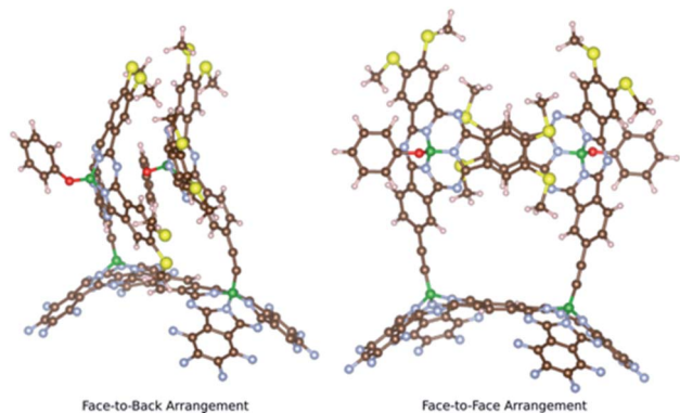
Fig. 1 Two computationally optimized structures of syn -SubPc 1.
