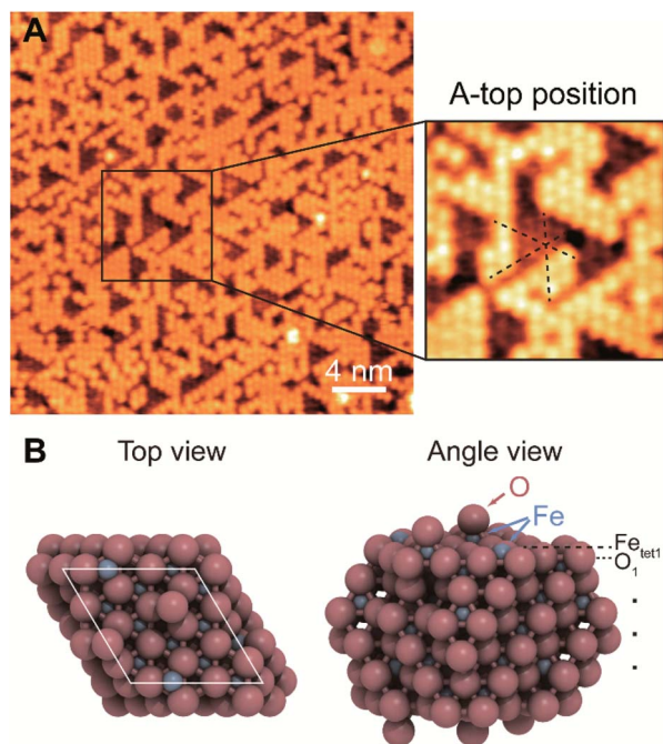
Fig. 1 The atomic-scale structure of Fe 3 O 4 (111)/ \alpha -Fe 2 O 3 (0001) is determined using: (A) an STM image of an oxygen adatom terminated Fe 3 O 4 (111) film, and (B) the corresponding DFT slab models with O adsorption coverage of 0.67 ML. The insert in (A) is a magnified image with close-packed directions of substrate indicated in black dashed lines. Scanning conditions: -1.5 V, 0.02 nA.
