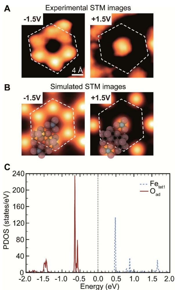
Fig. 2 Identification of oxygen adatoms and uncovered Fe tet1 by their distinct electronic states. (A) Experimental STM images showing a bias-dependent contrast change. (B) Simulated STM images based on DFT calculations. (C) DFT calculated site-projected density of states (PDOS) of oxygen adatoms (O ad ) and uncovered Fe tet1 atoms on the top layer. The PDOS includes both spin up and spin down components (i.e. not spin-resolved). The Fermi level is shifted to 0.0 eV. Experimental tunnelling current was 0.25 nA; probing bias was indicated in each panel. The regions encompassed by the dashed lines on the DFT model are a visual guide.
