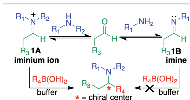
Fig. 2 Proposed high reactivity and selectivity towards secondary amines compared to primary amines.
