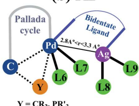
Fig. 2 A generalized representation of (a) concerted metalation–deprotonation (CMD) and (b) reductive elimination (RE) transition states with monometallic and heterobimetallic catalysts. 41 Only the most preferred ligand combinations, obtained by considering a much larger set of possibilities, are shown here. Details of various configurations considered are provided in Section 6 of the ESI. †
