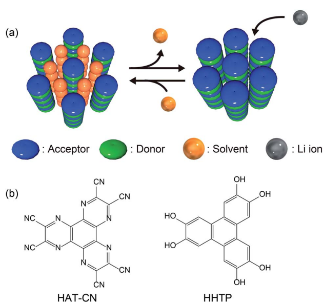
Fig. 1 (a) Schematic illustration of the proposed design strategy for redox-active porous structures using CT complexes. (b) Chemical structures of HAT-CN (acceptor) and HHTP (donor).
