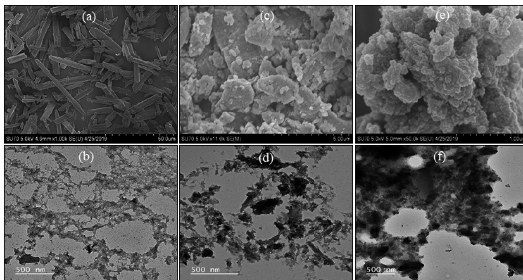
Fig. 8 SEM (top) and TEM (bottom) images of (a and b) MP, (c and d) ZrP, and (e and f) M-ZrP.
