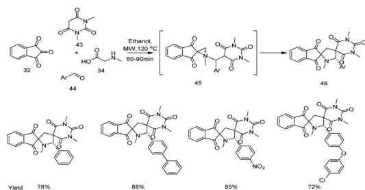
Scheme 15 Microwave mediated synthesis of regioselective diisopirrolidine analogs.
