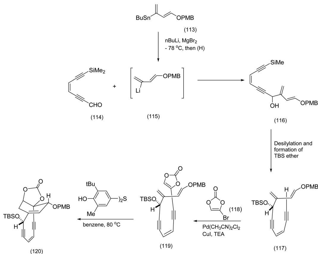
Scheme 28 Installation of the cyclic enecarbonate into the endiynone tethered. 88
