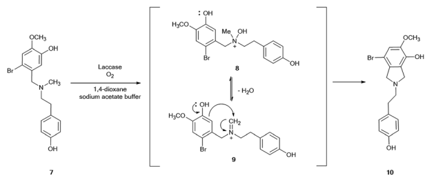
Scheme 3 Proposed mechanism for the laccase-mediated synthesis of isoidoline 10 starting from N -methyl-2-bromo- O -methylnorbelladine 7 .
