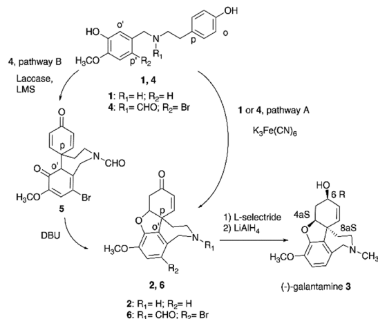
Fig. 1 Synthesis of galantamine 3. Pathway A: synthesis of galantamine 3 from O-methylnorbelladine 1 or N-formyl-2-bromo-O-methylnorbelladine 4 by use of K_3Fe(CN)_6 . Pathway B: laccase mediated synthesis of galantamine 3 from N-formyl-2-bromo-O-methylnorbelladine 4. LMS: laccase mediator system. DBU: 1,8-diazabicyclo [5.4.0]undec-7-ene.
