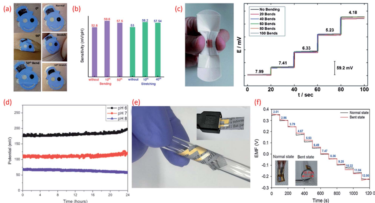
Fig. 5 (a) Images of the tattoo pH sensor with PANi sensitive electrode applied to cubital fossa at 0° bending, 90° bending, and after the 50th bending and stretching and images at normal, during stretching, and after the 10 th stretch. Reprinted with permission from Publication. 210 (b) The comparison of sensitivity variation of the tattoo-based sensors under different bending and stretching conditions. Reprinted with permission from Publication. 210 (c) Image of a bandage-based pH sensor with PANi electrode in bending condition and its calibration curves from pH 7.99 to 4.18 (each trace taken after 20 bends). Reprinted with permission from John Wiley and Sons. 152 (d) Long-term potential stability of the wound monitoring pH sensors (based on PANi electrode) at pH 6, pH 7 and pH 8 (pH values observed during chronic wound healing). Reprinted from Publication 206 with permission from Elsevier. (e) Image of a USB-type sensing platform and flexible state of an ion-selective sensor. Reprinted from Publication 134 with permission from Elsevier. (f) Response of pH sensors (PANi electrode) with increasing pH levels under mechanically normal and bent states (image shown in inset). Reprinted from Publication 134 with permission from Elsevier.
