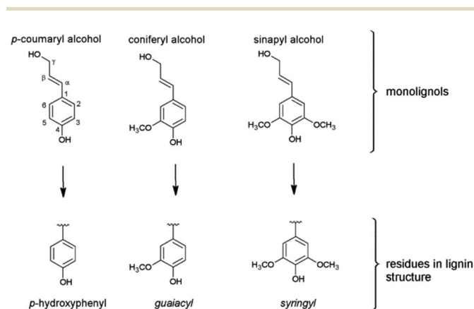
Fig. 1 The three monolignols and their corresponding structure units p -hydroxyphenyl (H), guaiacyl (G) and syringyl (S) of the lignin polymer.
