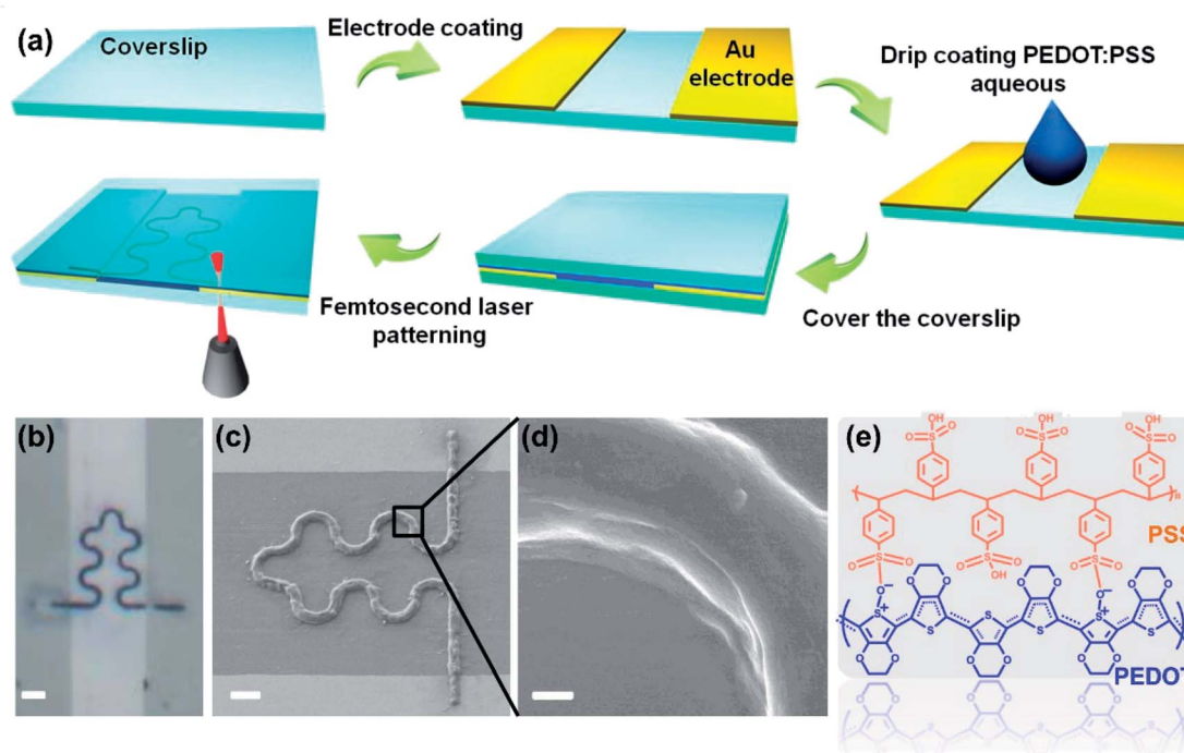
Fig. 1 (a) Fabrication schematic of the PEDOT:PSS micron line humidity sensor. (b) Optical microscope photograph of the PEDOT:PSS micron line humidity sensor (scale bar represents 10 μm). (c) SEM image of the S-shaped PEDOT:PSS micron line (scale bar represents 5 μm). (d) Zoomed in SEM image of the bend portion in the PEDOT:PSS micron line (scale bar represents 500 nm). (e) Molecular structure of PEDOT:PSS.
