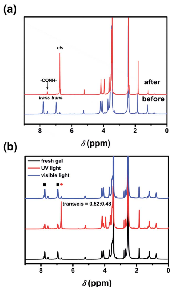
Fig. 5 (a) ^1\text{H} NMR spectra of Azo-mLCP in d_8 -dioxane before (bottom) and after UV irradiation (365 nm, 0.28\text{ mW cm}^{-2} ) for 10 min (top). (b) ^1\text{H} NMR spectra compositions of the gel based on Azo-mLCP (bottom), after UV light irradiation (middle), and subsequent irradiation under visible light (top). The black squares and the red circle represent the proton peaks of trans - and cis -isomer of azobenzene, respectively. The gel is prepared in d_8 -dioxane at a concentration of 7.5 wt%.
