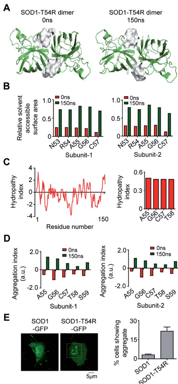
Fig. 8 Exposure of the R54-loop towards aqueous environment makes SOD1 T54R aggregation-prone. (A) Position of the surface of R54-loop of SOD1 T54R during different time points of simulation. (B) Solvent [water] accessibility of the residues of R54-loop of SOD1 T54R in the early and late phases of MDS. (C) Hydropobicity of the residues of SOD1 T54R . (D) Aggregation propensities of the residues of R54-loop during different time points of MDS. (E) Fluorescence microscopy image of expression and aggregation of SOD1 T54R -GFP in IMR-32 cells [yellow box represents aggregates of SOD1 T54R ].
