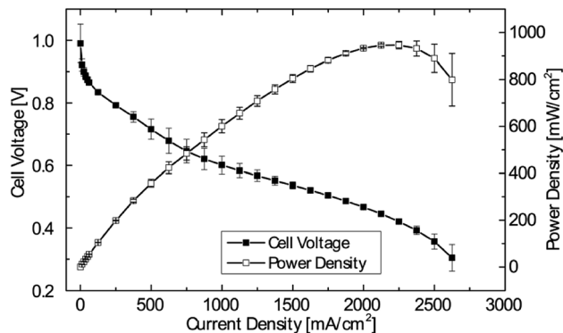
Fig. 4 Mean with error bars of polarization curves and power density curves of 3 DMD cells with 5 μm membranes. Operating conditions: anode/cell/cathode 69/70/70 °C, 0.5 slpm H 2 /O 2 , no back pressure. (For <62.5 mA cm -2 each measurement point held for 60 s, for ≥62.5 mA cm -2 each measurement point held for 90 s).
