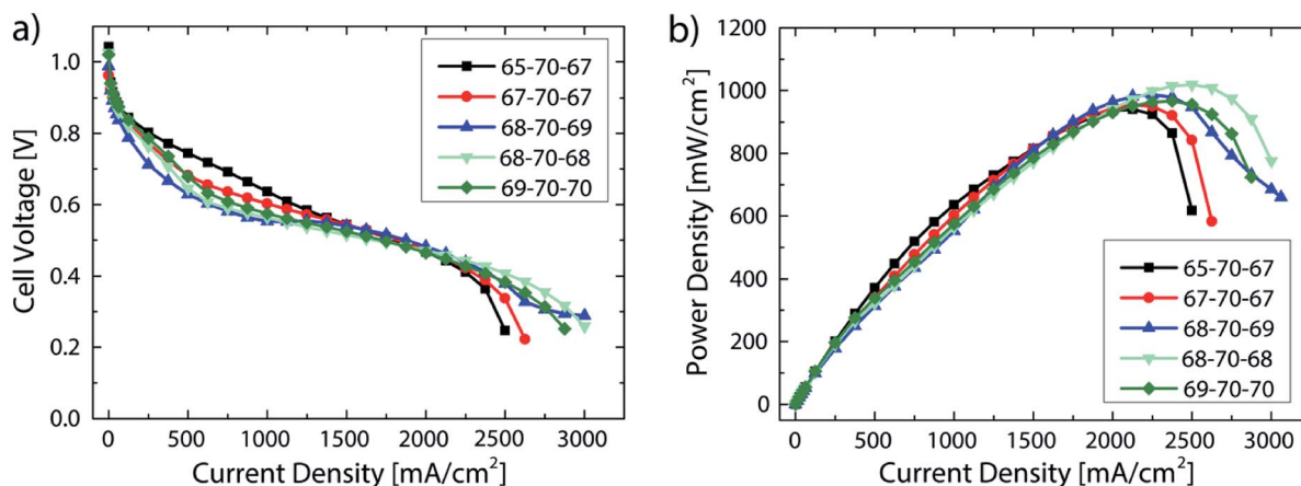
Fig. 5 Performance data of DMD cells with 5 μm membranes at varying relative humidity. The numbers given in the legend refer to the gas feed and cell temperatures: i.e. 65-70-67 refers to 65 °C anodic gas feed, 70 °C cell temperature, 67 °C cathodic gas feed. Operating conditions: 0.5 slpm H 2 /O 2 , no back pressure (a) polarization data, (b) power density data. (For <62.5 mA cm -2 each measurement point held for 60 s, for ≥62.5 mA cm -2 each measurement point held for 90 s).
