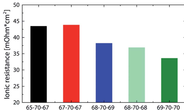
Fig. 6 Comparison of the ionic resistance (measured at 2 A cm -2 ) for DMD cells with 5 μm membranes at different gas feed dew points (corresponding performance data in Fig. 5). The numbers given in the legend refer to the gas feed and cell temperatures. i.e. 65-70-67 refers to 65 °C anodic gas feed, 70 °C cell temperature, 67 °C cathodic gas feed.
