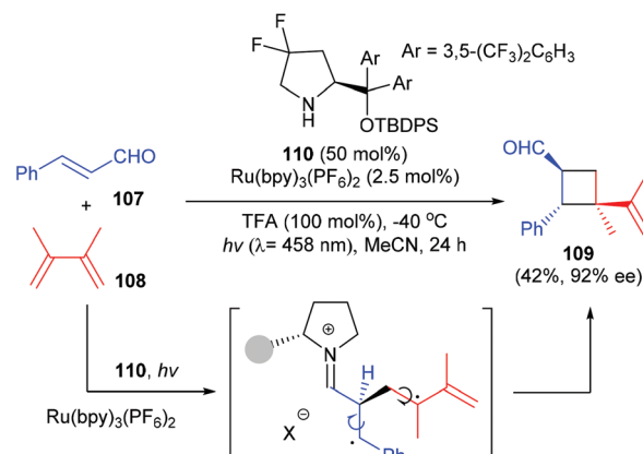
Scheme 31 Intermolecular [2 + 2] photocycloaddition of olefins with α,β-unsaturated aldehydes.
