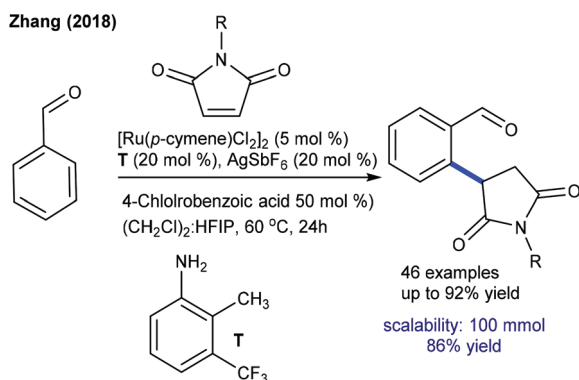
Scheme 58 ortho -Alkylation of aryl aldehydes with maleimides with a transient directing group.
