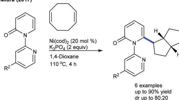
Scheme 51 C6-Selective ring-contracting C–H alkylation of 2-pyridones.
