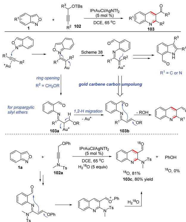
Scheme 40 Gold-catalysed C–H annulation of anthranils for the synthesis of quinoline derivatives.
