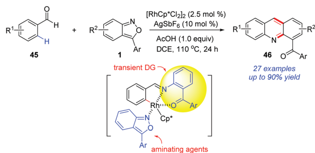
Scheme 16 Rh-Catalysed \text{C}(\text{sp}^2) -H amination of benzaldehydes with anthranils using a transient directing group strategy.
