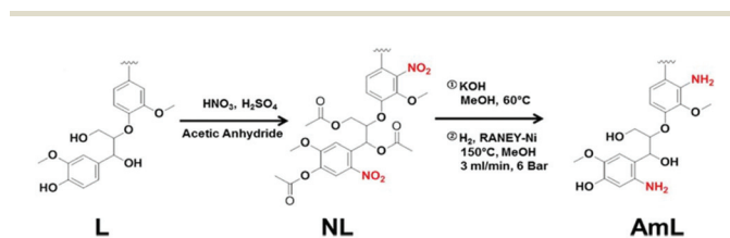
Fig. 2 Synthetic pathway for the conversion of alkali-lignin (L) into amino-lignin (AmL) via aromatic nitration.
