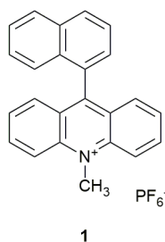
Fig. 2 10-Methyl-9-(1-naphthalenyl)acridinium hexafluorophosphate dyad that undergoes triplet formation by charge recombination from a charge-transfer state. 24
