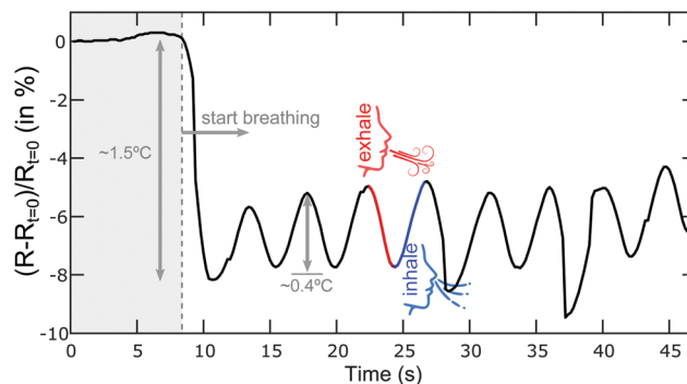
Fig. 6 Implementation of a respiration monitoring device using the WS 2 -on-paper thermal sensor. Resistance change vs. time of WS 2 thermal sensor device when a test person breaths at ~1 cm over the sensor (breathing starts at t \sim 8 s). The thermoresistive device resolves the inhaling/exhaling cycles because of a ~0.3–0.5 °C increase in the temperature of the sensor upon exhaling. Note: The sensor has been encapsulated with Scotch tape to reduce the effect of humidity changes during the breathing cycles on the resistance.
