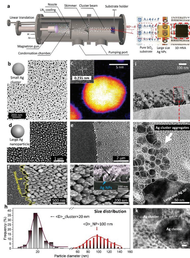
Fig. 2 (a) Left: Schematic illustration of the gas phase cluster beam deposition system. Right: Photographs of the blank \text{SiO}_2 substrate, large size Ag NP sample and 3D-HNA sample. (b) TEM image of Ag clusters generated from the cluster deposition system. (c) Typical HAADF-STEM image of a single Ag cluster. The inset is the HR-STEM image of the Ag cluster and the corresponding lattice constant has been marked in the figure. (d) SEM image of large size Ag NPs from the solid-state film dewetting process. (e) A typical SEM image of Ag cluster assemblies (left part) and 3D-Ag-HNA (right part). (f) A high magnification SEM image of Ag cluster assemblies (left part) and 3D-Ag-HNA (right part), the shadowing region has been marked in the figure. The inset shows a typical cross-sectional SEM image of 3D-Ag-HNA. (g) A high magnification SEM image of 3D-Ag-HNA. The inset shows a high magnification cross-sectional SEM image of 3D-Ag-HNA. (h) Size distribution of the Ag nanoparticles in the 3D-Ag-HNA and the corresponding log-normal fits. (i) TEM image of 3D-Ag-HNA. (j) A high magnification cross-sectional TEM image of a single unit in the 3D-Ag-HNA structure. (k) A high magnification TEM image of two Ag nanoclusters in the aggregate.
