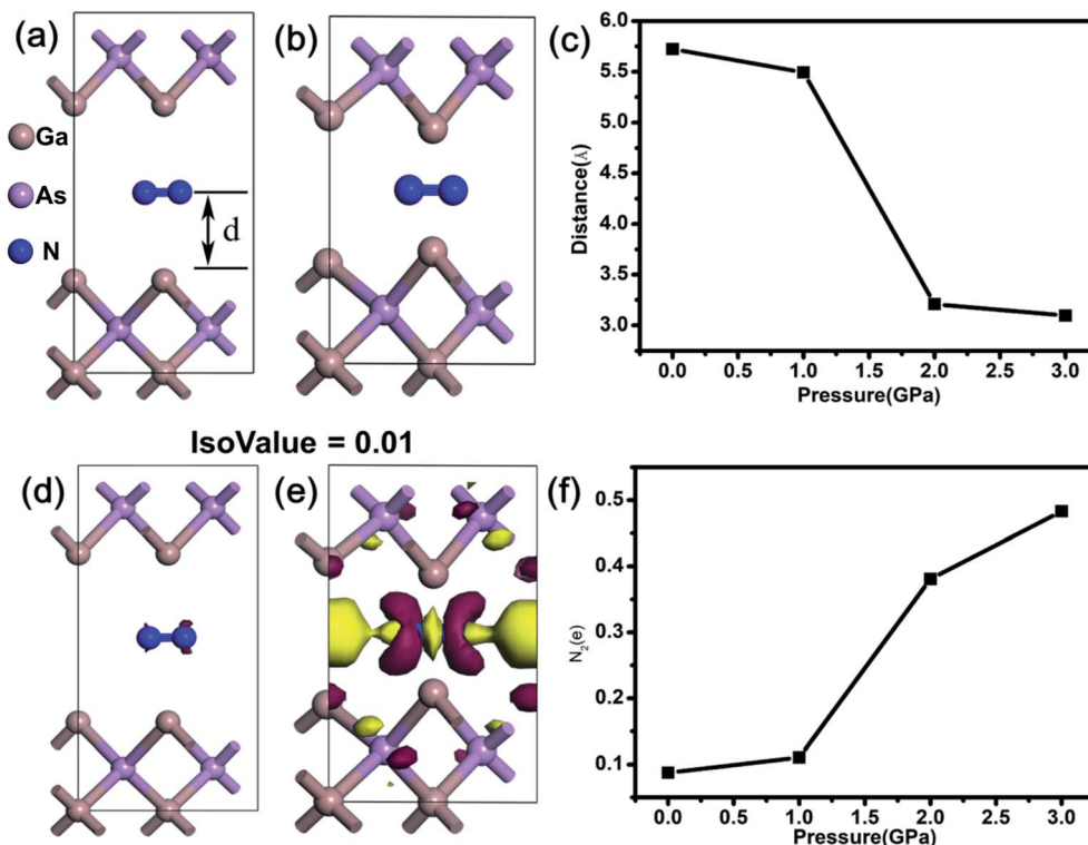
Fig. 4 (a) N_2@GaAs unit cell model at 0 GPa. d is the distance between the nitrogen molecule and the GaAs layer. (b) N_2@GaAs unit cell model at 2 GPa. (c) Distance–pressure curve of selected pressure (0 GPa, 1 GPa, 2 GPa and 3 GPa). (d) Electron density difference of N_2@GaAs at 0 GPa with an isovalue of 0.01. (e) Electron density difference of N_2@GaAs at 2 GPa with an isovalue of 0.01. The purple and yellow colors indicate electron accumulation and electron depletion, respectively. (f) Transferred charge quantity as a function of pressure.
