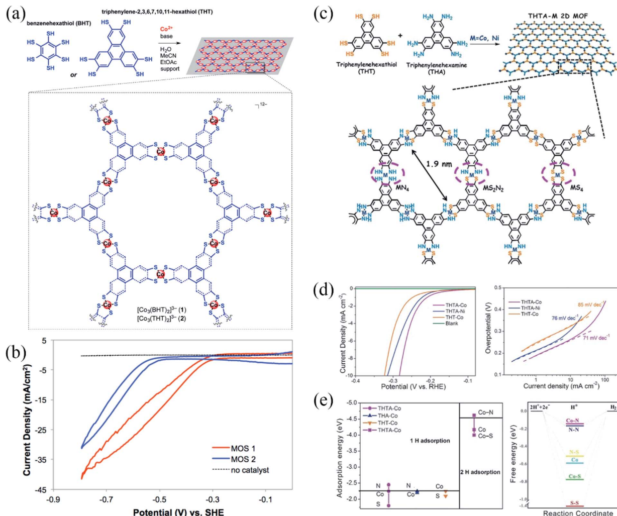
Fig. 18 (a) Synthesis of cobalt dithiolene films, Co-BHT and Co-THT, the films are deposited onto the desired supports, generating \text{MOS}_1 and \text{MOS}_2 ; (b) polarization curves of \text{MOS}_1 (red) and \text{MOS}_2 (blue) at pH 1.3, scan rate, 100 \text{ mV s}^{-1} ; reproduced with permission. 162 Copyright©2015 American Chemical Society. (c) The synthesis of single-layer 2D MOFs, in which \text{MS}_2\text{N}_2 complexes along with \text{MN}_4 and \text{MS}_4 moieties were incorporated into the hexagonal networks through metal dithiolene–diamine coordination (THTAM) ( \text{M} = \text{Co} and \text{Ni} ); (d) HER polarization plots (left) of three types of 2D MOFs: THTA-Co (purple), THTA-Ni (blue), and THT-Co (yellow) and a blank glassy carbon disk electrode in 0.5 \text{ M H}_2\text{SO}_4 and the Tafel plots (right) obtained from the polarization curves; (e) the adsorption energy of one H and two H radicals bonding to the proposed active sites on the surface of THTA-Co, THA-Co, and THT-Co 2D MOFs (left) and the free-energy diagram of the HER at the equilibrium potential for the THTA-Co 2D MOFs with the possible active sites (right). Reproduced with permission. 144 Copyright©2017 WILEY-VCH Verlag GmbH & Co. KGaA.
