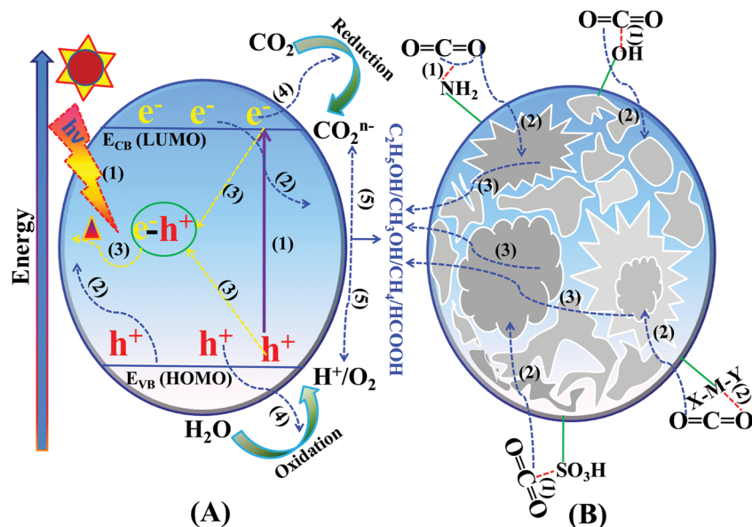
Scheme 12 Basic mechanism of the photocatalytic process: (A) optoelectronic steps and (B) physicochemical steps involved in the \text{CO}_2 reduction reaction.
