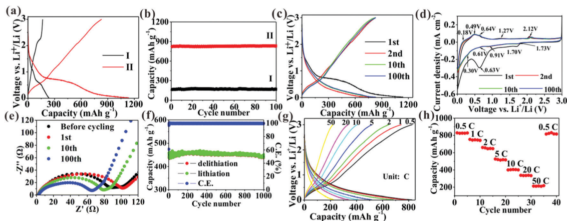
Fig. 5 (a) First charge/discharge curves; (b) cycling curves at 0.5C of TiO₂/C (I) and SnO₂@TiO₂/C (II); (c) charge/discharge curves at different cycles; (d) CV curves; (e) Nyquist plots; (f) cycling performance at 10C; (g) charge/discharge curves at different current densities; and (h) rate performance of SnO₂@TiO₂/C.
