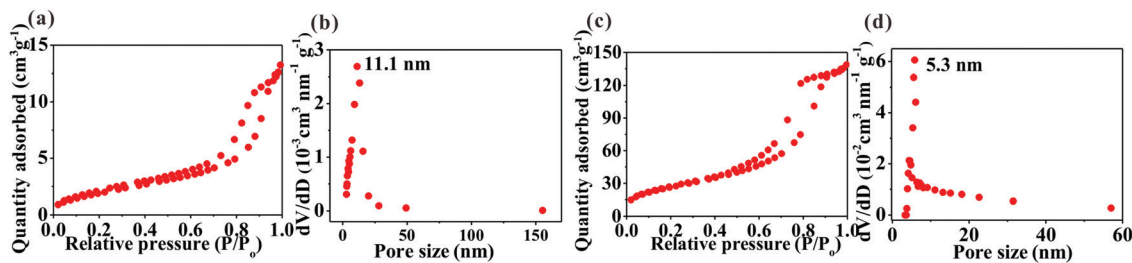
Fig. 4 Nitrogen adsorption-desorption isotherms and pore-size distribution of TiO₂/C (a and b) and SnO₂@TiO₂/C (c and d).
