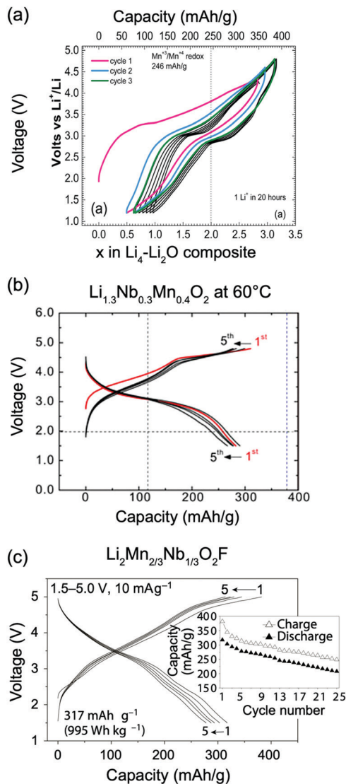
Fig. 15 Electrochemical performance of selected Mn redox-based DRX cathodes. Room temperature electrochemical profiles of the nanostructured (a) 0.93Li 3.6 Mn 2.4 O 5.4 -0.07Li 2 O composite, when cycled between 1.2 and 4.8 V. Figure adapted from Freire et al. 64 with permission from the Royal Society of Chemistry. (b) Electrochemical profile of Li 1.3 Nb 0.3 Mn 0.4 O 2 at 60 °C, when cycled between 1.5 and 4.8 V. Figure adapted from Yabuuchi et al. 13 with permission from PNAS. (c) Room temperature electrochemical profile of Li 2 Mn 2/3 Nb 1/3 O 2 F, when cycled between 1.5 and 5.0 V. Adapted by permission from Springer Nature: Lee et al. , 20 copyright 2018.
