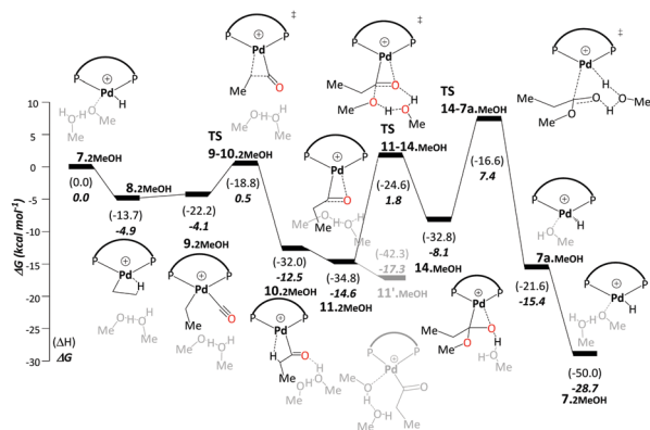
Scheme 5 Hydride-hydroxyalkylpalladium pathway C : free energy profile using methanol as the model solvent at the B3PW91-D3/ECPC/PCM level. Energies are in kcal mol -1 relative to 7.2MeOH . Explicit solvent molecules are shown in light grey colour. Final free energies \Delta G and enthalpies ( \Delta H ).
