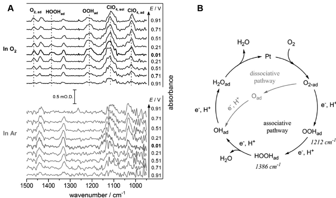
Fig. 12 (A) ATR-IR spectra on Pt/C nanoparticle during ORR and under Ar in 0.1 M \text{HClO}_4 . The reference spectra are obtained at 1.01 V vs. SHE. (B) Proposed mechanism of ORR at a Pt/C nanoparticle catalyst in 0.1 M \text{HClO}_4 . The figure and caption were adopted from the reference with permission from the ref. 201. Copyright (2018) Wiley-VCH.
