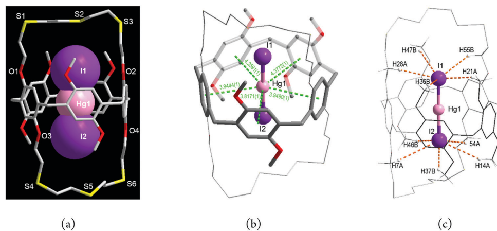
Fig. 4 The contact ion-triplet complex with mercury(II) iodide [\text{I}(\text{HgI})@L] ( 3 ): (a) general view showing an (\text{I}^- - \text{Hg}^{2+} - \text{I}^-) entity (space-filling) in the central cavity, (b) a pentagonal bipyramidal geometry with five \text{Hg}^{2+}\cdots\pi interactions (green dashed lines) and an \text{I}-\text{Hg}-\text{I} axis and (c) a mercury-shared double pentagonal pyramidal geometry with five \text{C}-\text{H}\cdots\text{I}^- H-bonds (orange dashed lines) and \text{I}-\text{Hg}-\text{I} axis (only H-bonded H atoms are shown).
