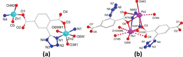
Fig. 1 Coordination environments of the \text{Zn}(\text{II}) ions and \text{Pb}(\text{II}) ions in 1 (a) and 2 (b); symmetry codes for 1: #1: 2 - x, 1 - y, 1 - z and #2: 1.5 - x, 0.5 + y, 0.5 - z ; for 2: #1: 1 - x, 1 - y, 1 - z ; #2: -x, -y, 2 - z ; #3: x - 1, y, z ; #4: x, 1 + y, z ; #5: x, y - 1, z ; and #6: 1 - x, -y, 2 - z .
