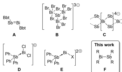
Scheme 1 Isolated compounds containing Bi–Sb bonds. See text for references. Bbt = o,o -( \text{CH}(\text{SiMe}_3)_2 )- p - \text{C}(\text{SiMe}_3) -Ph.
