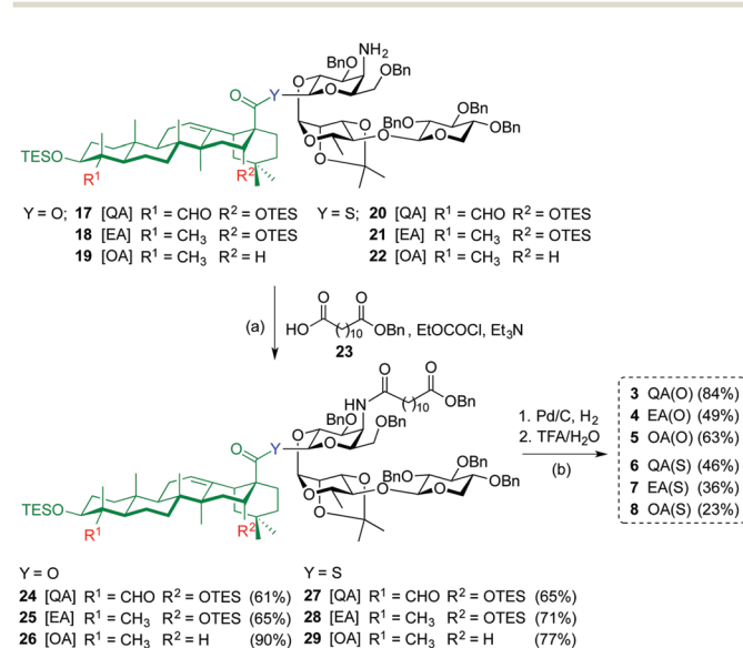
Scheme 2 Reagent and conditions: (a) \text{EtOCOC}_8\text{OBn} , \text{Et}_3\text{N} , THF, 0 °C to r.t., 4 h, 61% (for 24 ), 65% (for 25 ), 90% (for 26 ); 65% (for 27 ), 71% (for 28 ), and 77% (for 29 ); (b) 1: Pd/C, \text{H}_2 (1 atm), \text{EtOH}/\text{THF} 1 : 1, r.t., 16 h (for 24–26 ); 20 min (for 27–29 ); 2: TFA/ \text{H}_2\text{O} 3 : 1, 0 °C, 1 h, 84% (for 3 ), 49% (for 4 ), 63% (for 5 ); 46% (for 6 ), 36% (for 7 ), and 23% (for 8 ).
