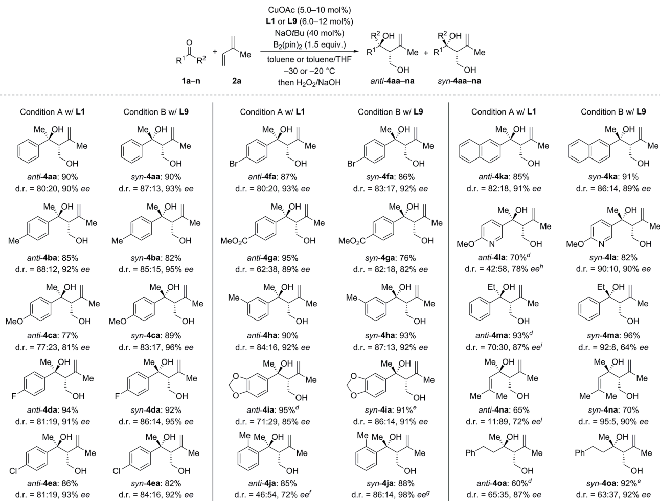
Scheme 2 Scope I: variation the ketone. a–c Condition A: CuOAc (10 mol%), L1 (12 mol%), NaOtBu (40 mol%), ketone 1 (0.20 mmol), isoprene ( 2a , 1.0 mmol), and B 2 (pin) 2 (1.5 equiv.) in toluene (2 mL) at –30 °C. Condition B: CuOAc (5.0 mol%), L9 (6.0 mol%), NaOtBu (40 mol%), ketone 1 (0.40 mmol), isoprene ( 2a , 2.0 mmol), and B 2 (pin) 2 (1.5 equiv.) in toluene/THF – 8 : 2 (3.5 mL) at –20 °C. b Yields are combined isolated material; diastereomers are usually separable by flash chromatography on silica gel. c The enantiomeric excess of the major diastereomer was determined by HPLC analysis on chiral stationary phases. d CuOAc (15 mol%) and L1 (18 mol%) were used. e CuOAc (10 mol%) and L9 (12 mol%) were used. f anti-4ja : 29% ee. g anti-4ja : 80% ee. h ee value of anti-4la . i syn-4ma : 78% ee. j syn-4na : 72% ee.
